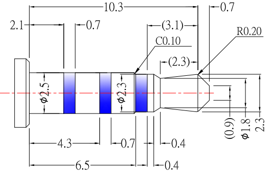
ø2.50mm 4 POLE PLUG DETAIL DRAWING
